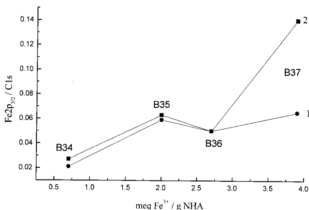
Fig. 4 Dependency of the relative \text{Fe2p}_{3/2}/\text{C1s} line intensity on the relative concentration meq \text{Fe}^{3+} /g NHA of the complexes. Curve 1 (circles) – powdered samples (bulk); curve 2 (squares) – non-powdered samples (surface).
