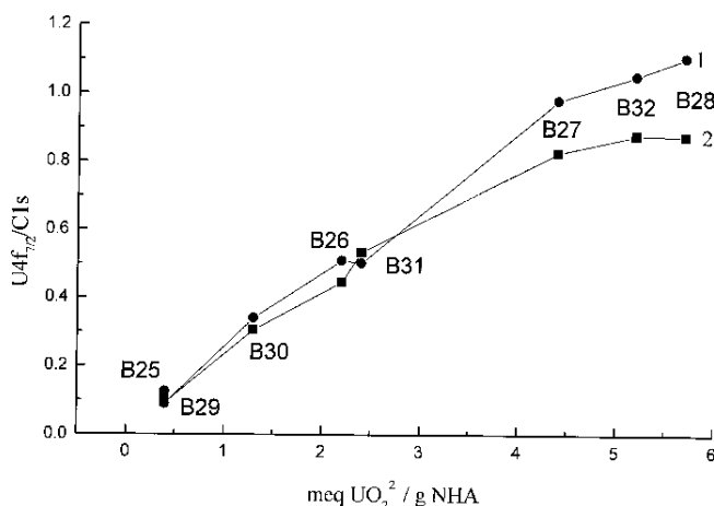
Fig. 3 Dependency of the relative \text{U4f}_{7/2}/\text{C1s} line intensity on the relative concentration meq \text{UO}_2^{2+} /g NHA of the complexes. Curve 1 (circles) – powdered samples (bulk); curve 2 (squares) – non-powdered samples (surface).
